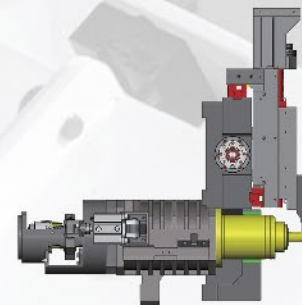
Y1轴刀架采用龙门式L型排布 Y1 axis tool rest adopts gantry type L-type layout
